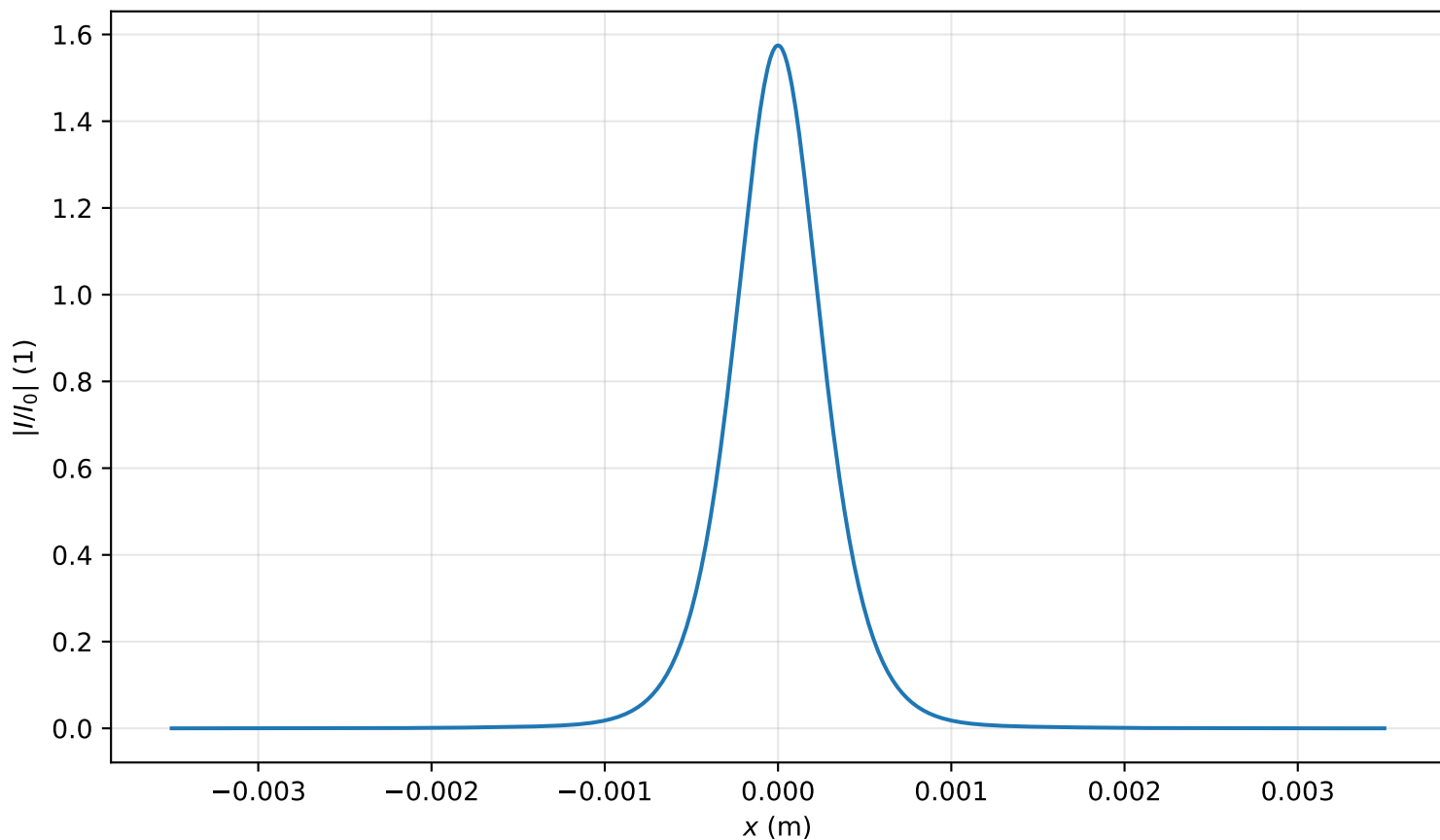
Intensity profile I(x, y = 0, z = 2.946m)/I_0 , P_{in}=0.9P_{cr} , artificial time
